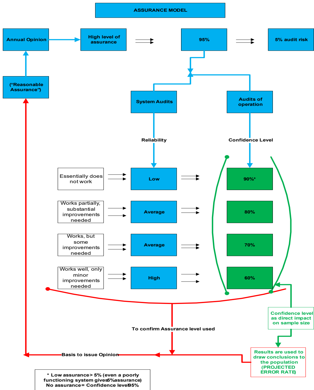
Figura 16 - Assurance model
